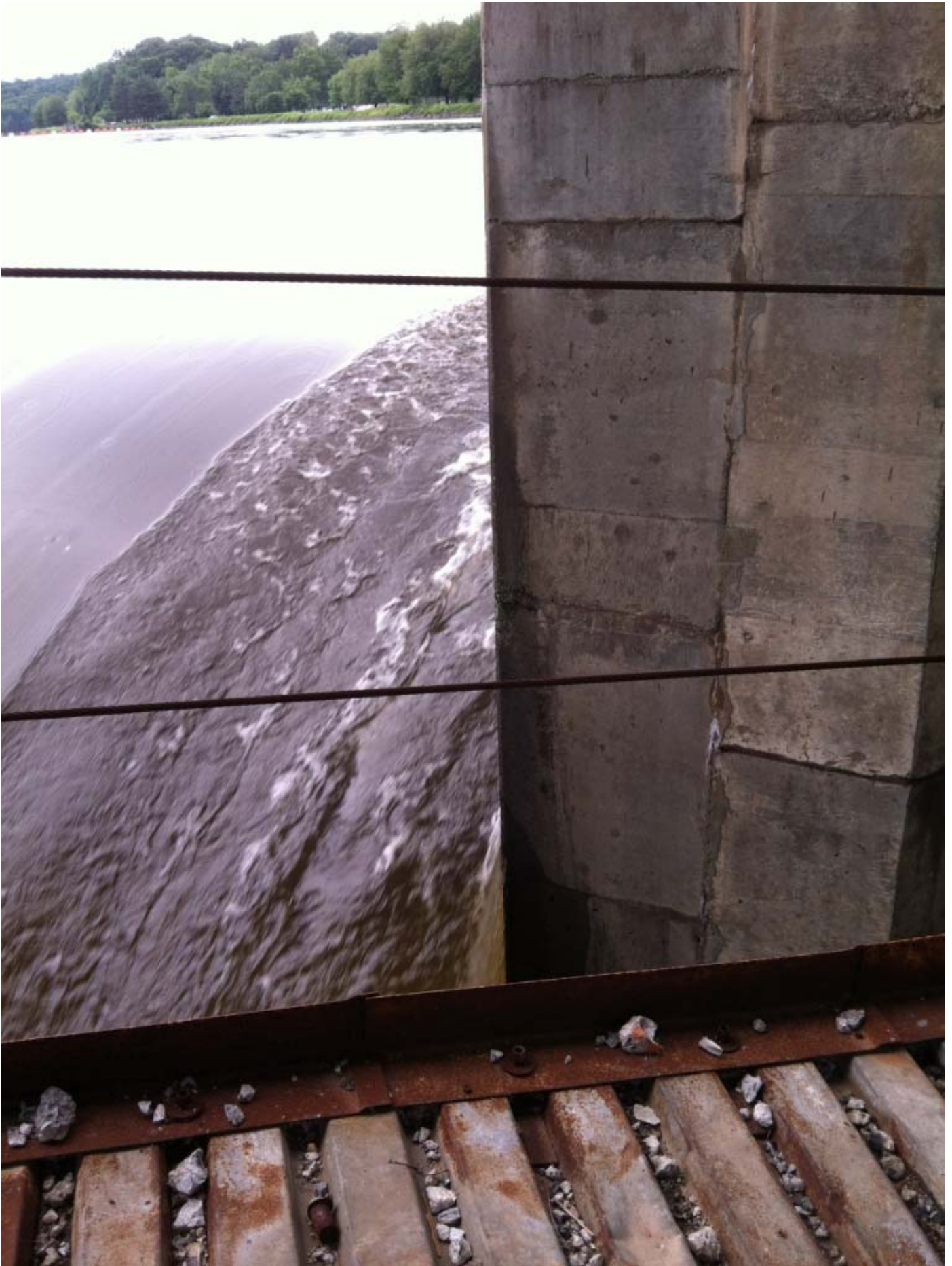
Lower Cable/Metal Deck Platform Below Bottom Truss Chord
